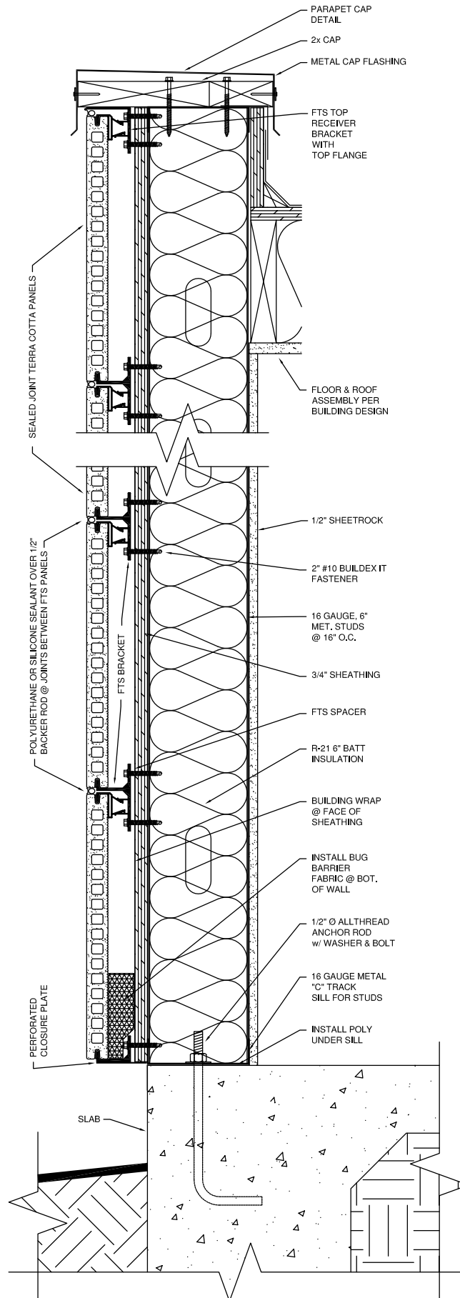
SEALED JOINT TERRA COTTA PANEL INSTALLATION
