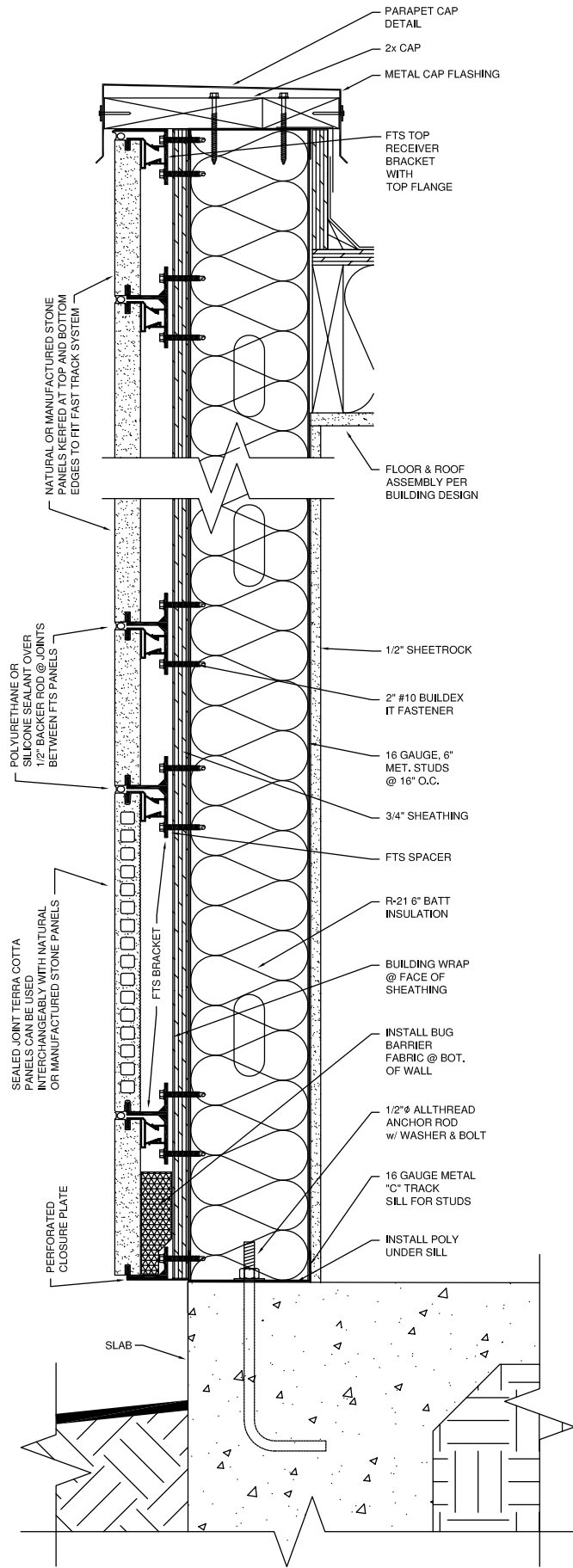
SEALED JOINT STONE/TERRA COTTA PANEL INSTALLATION
