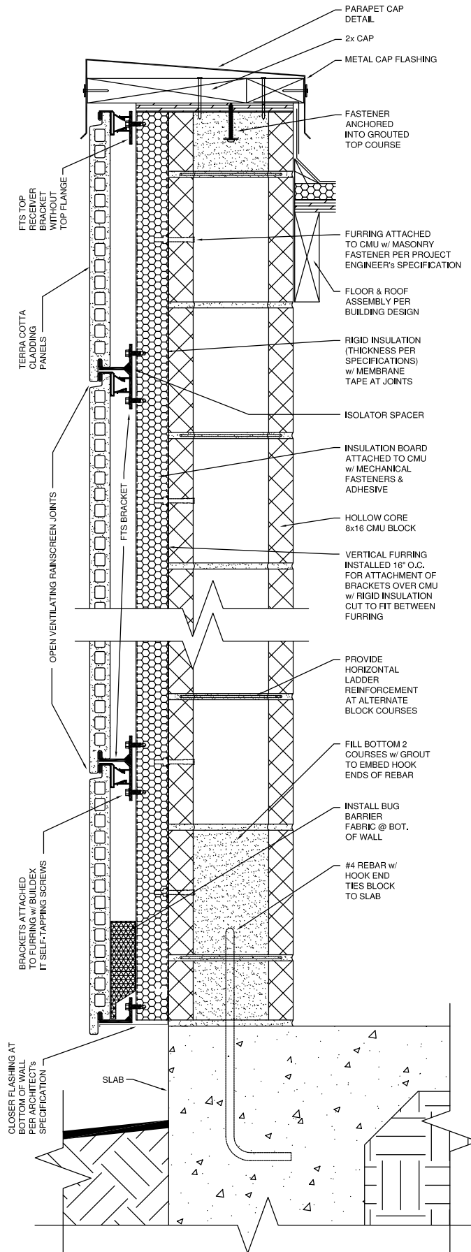
OPEN JOINT TERRA COTTA RAINSCREEN PANEL INSTALLATION
